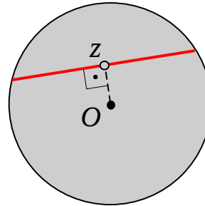
p -line (invariant principle)
